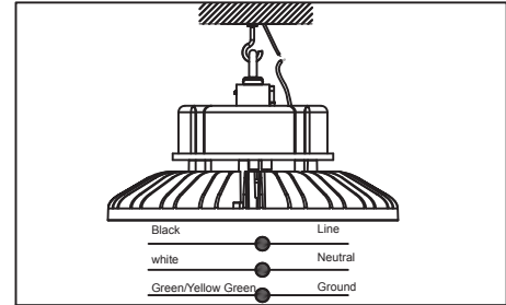
3. Connect the three wires (L: Black N: White G: Green) with the correct cable as shown in the figure.
