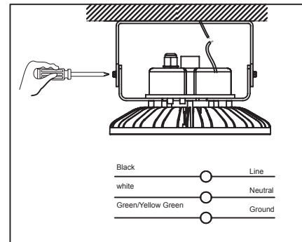
3. Adjust UFO fixture to correct position, fasten the screw. Connect to AC wire.
