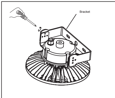
1. Use tools to screw out the screws at both ends of the bracket. (as shown in the figure)
