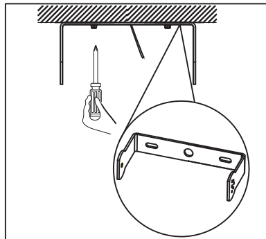
2. The bracket is fixed to the ceiling with two screws. (as shown in the figure)
