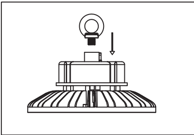
1. The suspension ring is assembled on the lamp body and the side anti-loosening screw is tightened.
