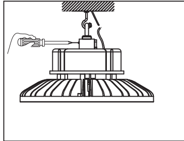
2. Hang the lamp hook on the lamp hook.
